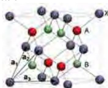
Figure 1 : the half Heusler structure
