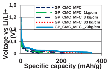
Figure 1b : Specific capacity as function of calendaring conditions.
