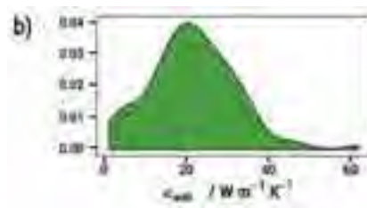
Figure 2B : Distribution of thermal conductivities throughout the stable compounds
