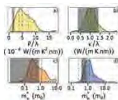
Figure 4 : Frequency distributions among the 77 HHs of: a) power factors b) total thermal conductivities divided by grain size c) effective masses of electrons and d) of holes. The shaded areas span the values of each variable among the other seven semiconductors
